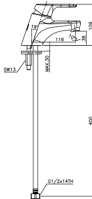
FRONT VIEW
