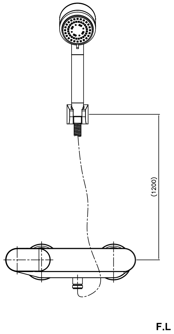
SIDE VIEW
