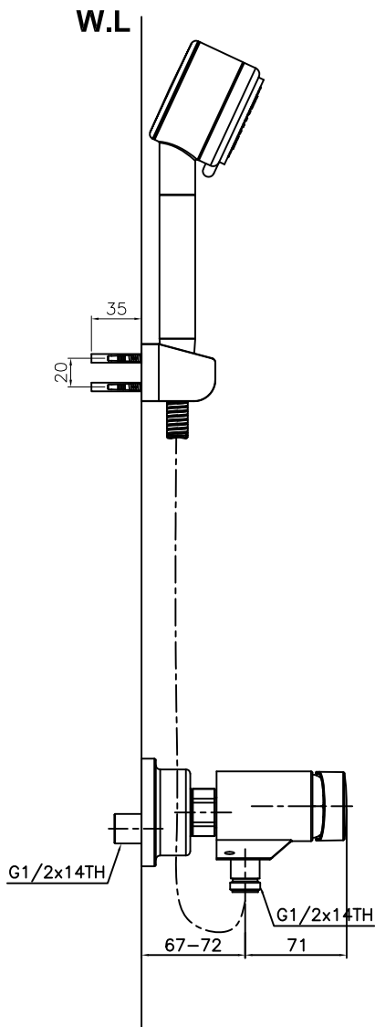
FRONT VIEW
