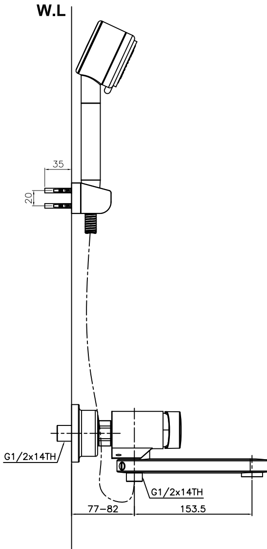
FRONT VIEW
