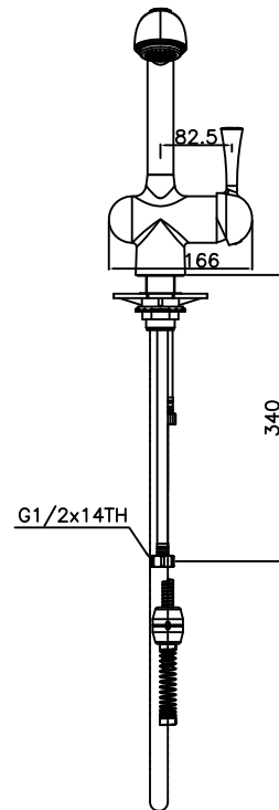
FRONT VIEW
