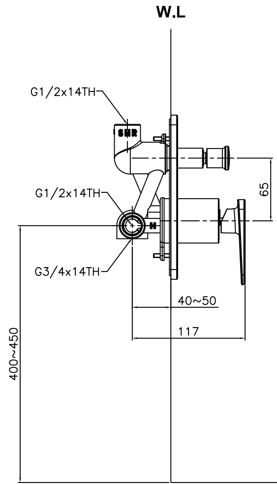
FRONT VIEW
